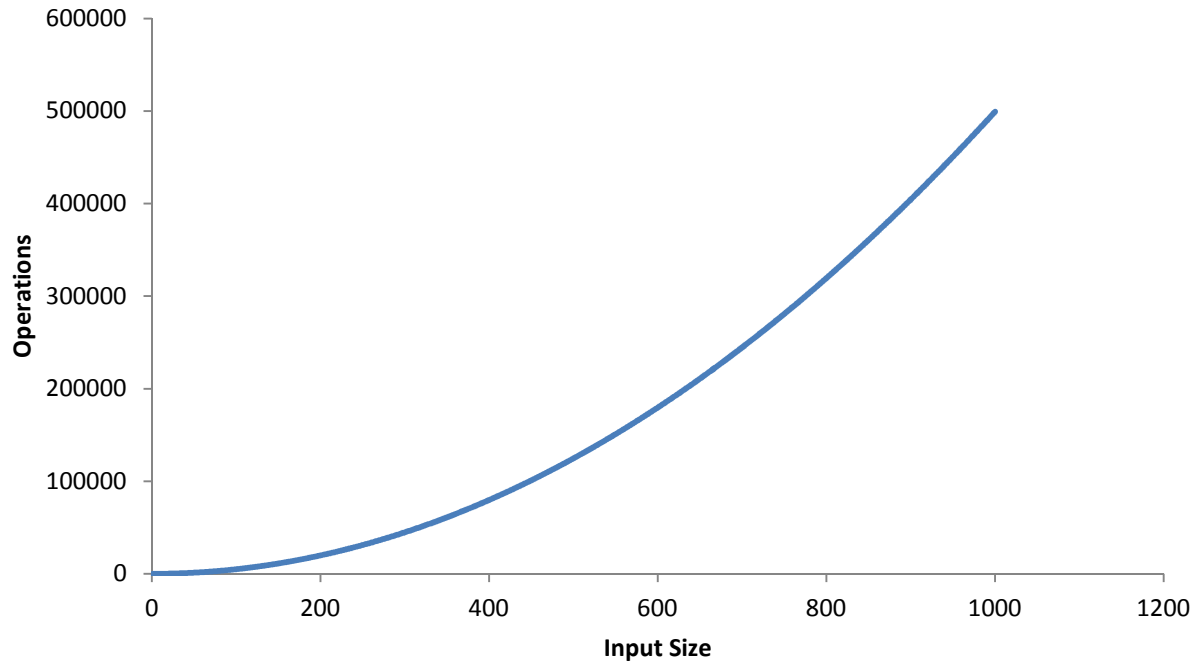
Insertion Sort
