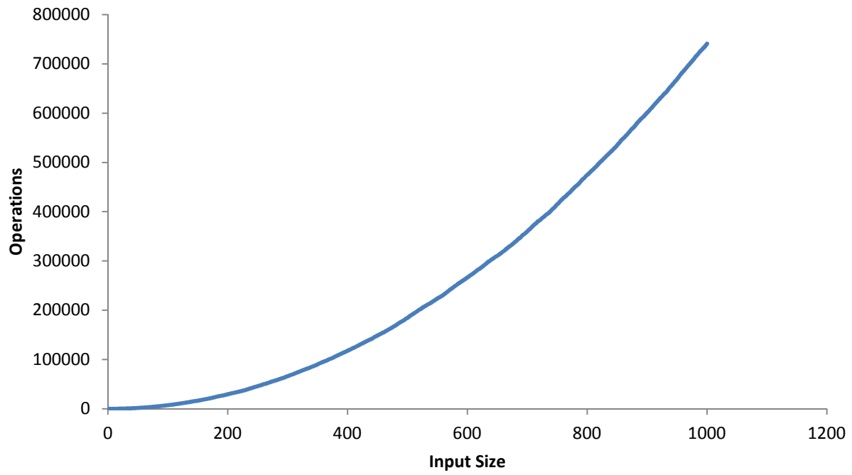
Selection Sort
